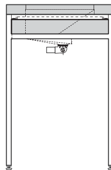
MODEL 9110...3670-RH... (Shown: Unit with Right Offset 3670 Deep Ebb Basin)
